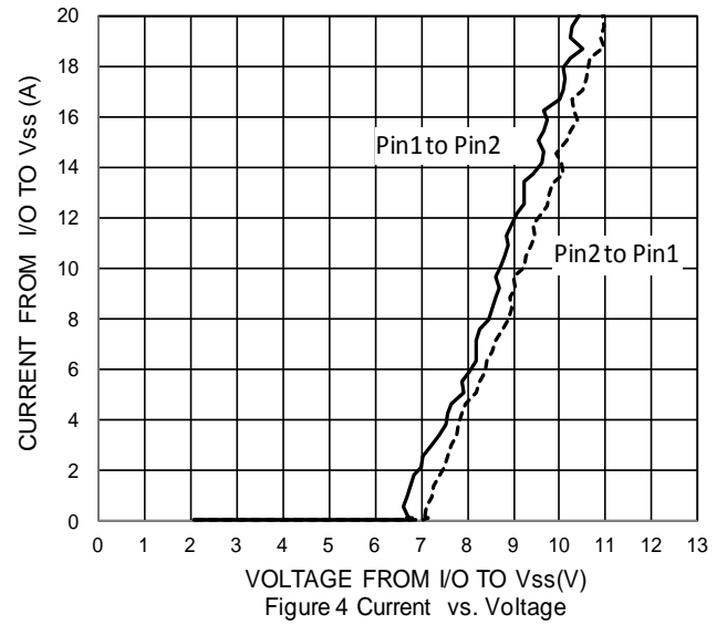
Figure 4 Current vs. Voltage
